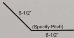
Rollform 92 J-Channel
