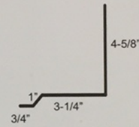
113 Inside Corner
