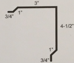
100 Sidewall
