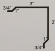
104 Residential Rake/Corner
