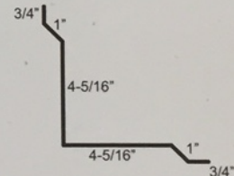
199 Drip Cap
