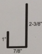
Rollform 92 J-Channel
