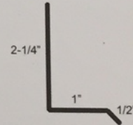
199 Drip Cap
