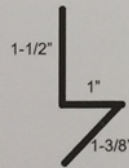
161 Angled Base
