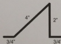
140 Pipe Guard
